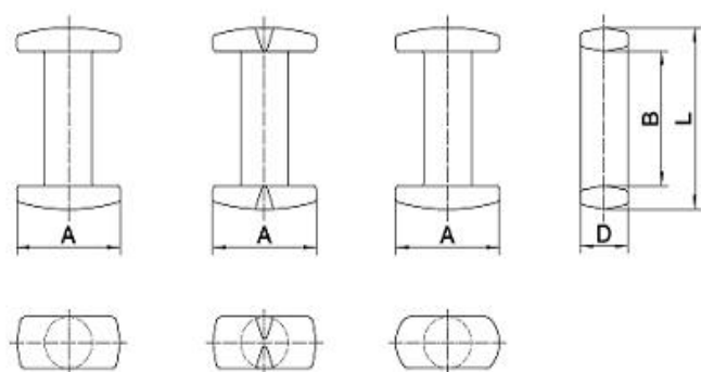
Regular Pin
