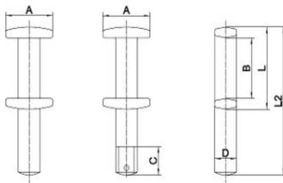
Extended Pin
