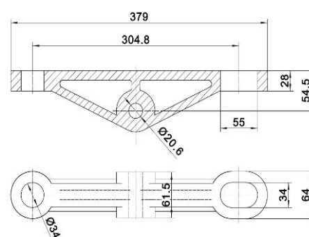
Load bar for X678 trolley
